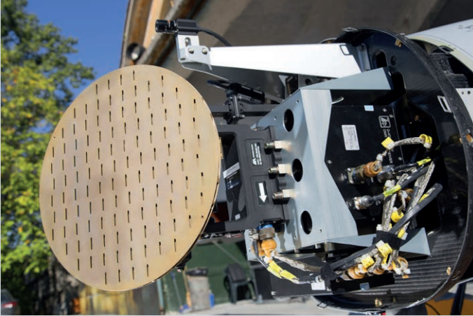
Surveillance Radar
